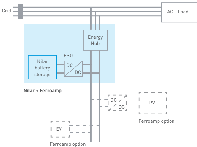
Nilar and Ferroamp solution configuration scheme
